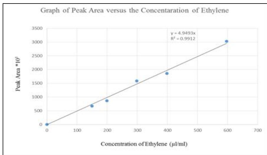
Figure 1: Graph of Peak Area versus the Concentrations of Ethylene standard as output from Shimadzu Gas Chromatograph.
